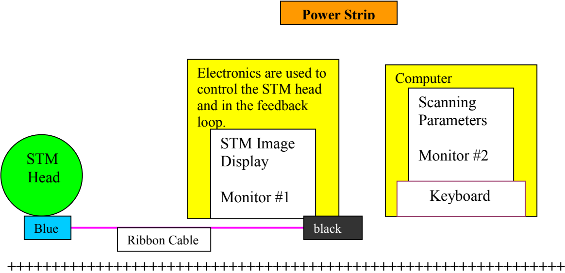
Set-up Diagram – Backview
