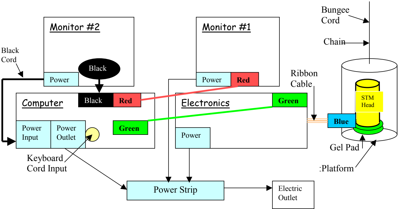
Set-up Diagram – Backview
