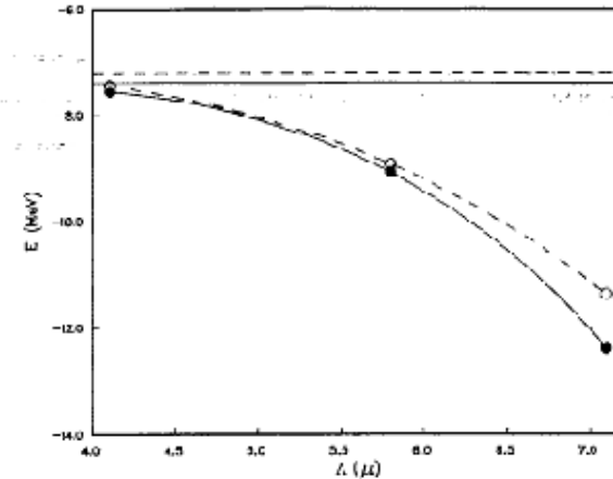
FIG. 1. Triton binding energy E obtained from 18-channel calculations vs the cutoff parameter \Lambda in the \pi NN form factor of the Tucson-Melbourne three-nucleon force. The horizontal lines correspond to results without three-nucleon force. The full circles are binding energies calculated actually with the Paris potential and the Tucson-Melbourne three-nucleon force; the empty circles are binding energies actually calculated with the RSC potential and the Tucson-Melbourne three-nucleon force. The solid and dashed curves through the circles are drawn to guide the eye.
