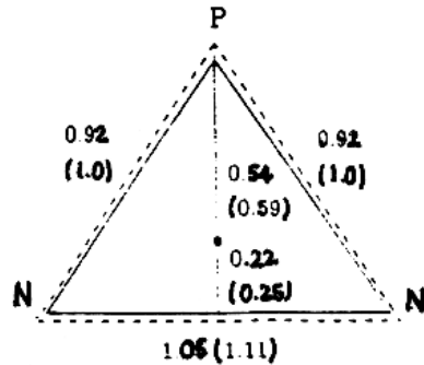
The most probable sites of protons and neutrons in {}^3\text{H} for the Paris (dashed) and the Bonn B (solid) potentials. Distances are given in fm for Bonn B and Paris (in parenthesis).
